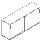
A2P16 1610 / 432 / 740 74.4 kg
